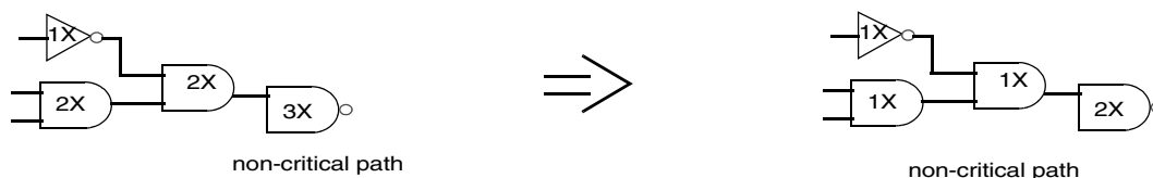
Figure 18-2 Example of Downsizing Cells During Area Recovery
