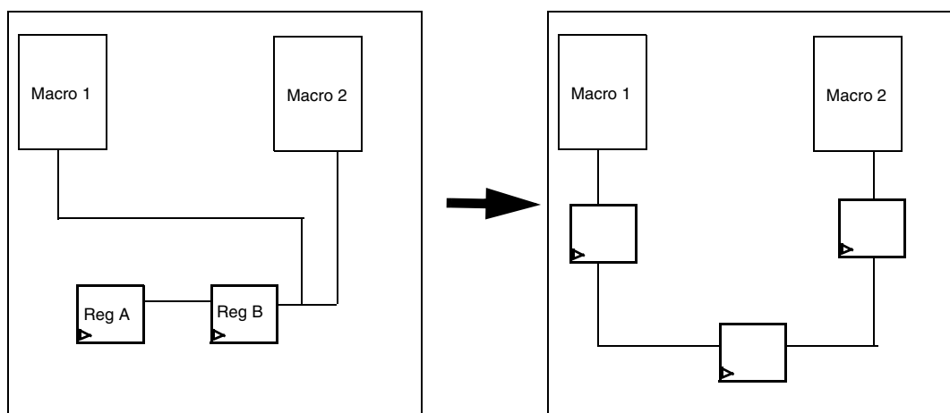
Figure 15-16 Register Replication Example
