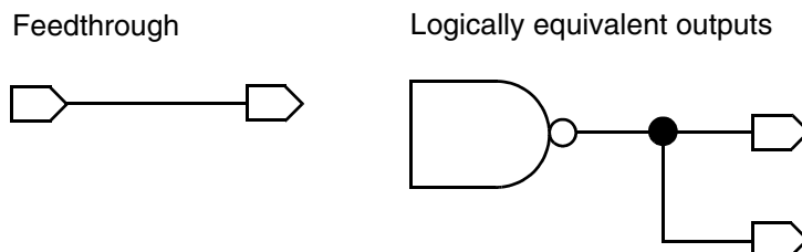
Figure 11-11 Multiple-Port Connection Types
