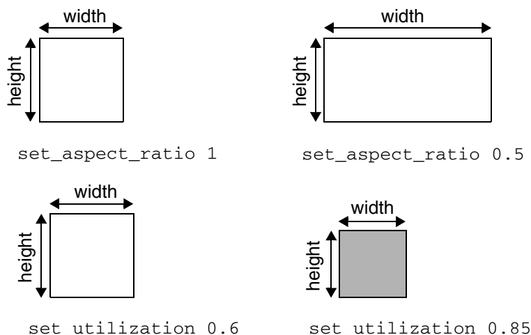
Figure 9-2 Using the set_aspect_ratio and set_utilization Commands
