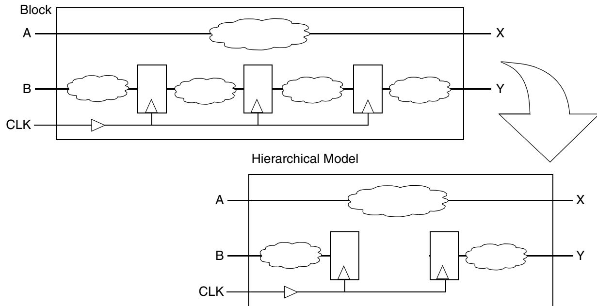
Figure 22-1 A Block and Its Hierarchical Model
