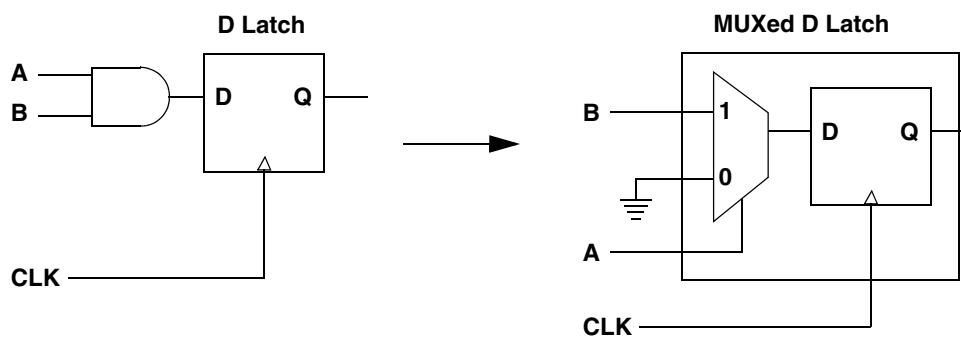
Figure 11-3 Sequential Optimization
