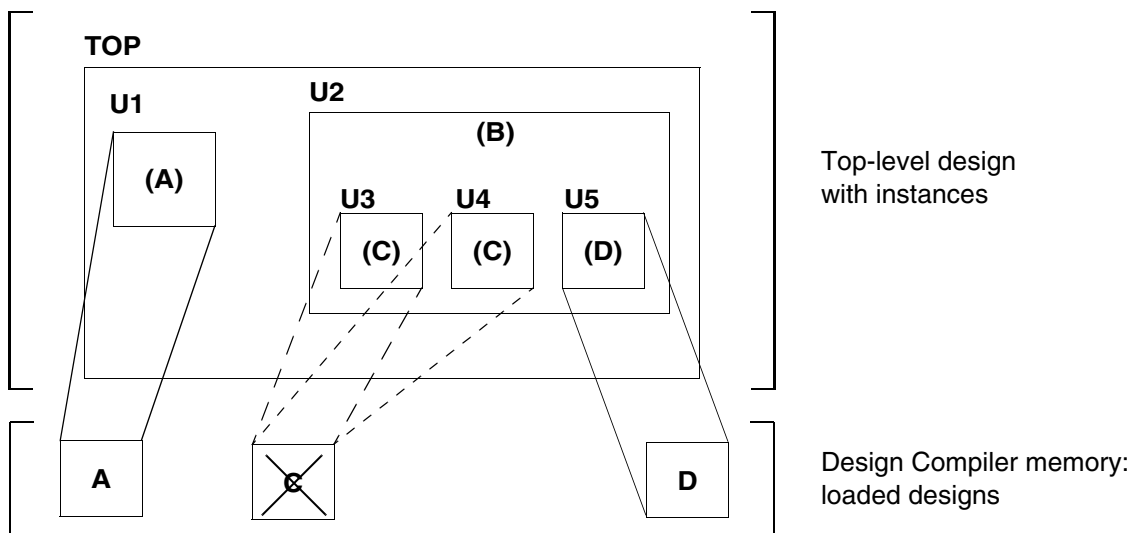
Figure 10-6 Compile-Once-Don't-Touch Results
