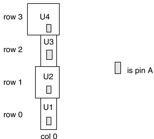
Figure 9-18 Relative Placement Group Aligned by Pins
