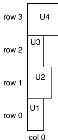
Figure 9-14 Bottom-Left-Aligned Relative Placement Group
