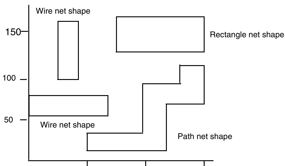
Figure 9-7 Types of Preroutes
