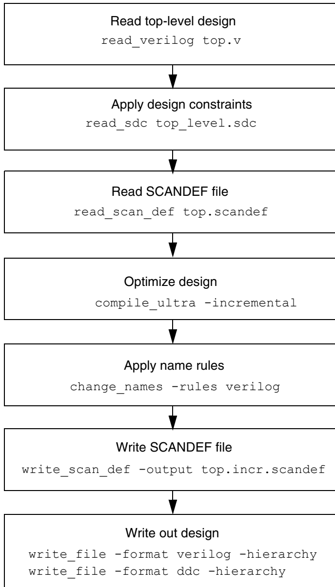
Figure 23-2 Netlist SCANDEF Flow Example
