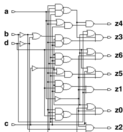
Figure 11-1 Logic-Level and Gate-Level Optimization for Design LED
