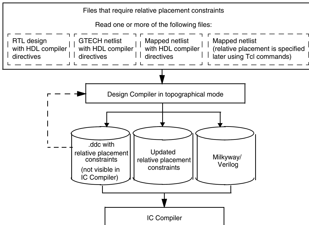
Figure 9-11 Relative Placement Flow
