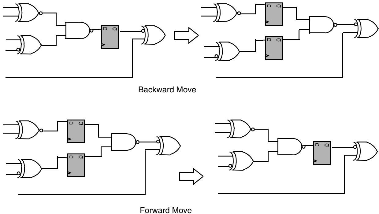
Figure 16-1 Adaptive Retiming
