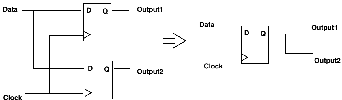
Figure 15-3 Merging Equal and Opposite Registers
