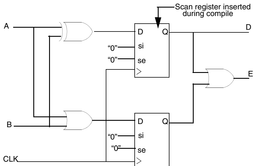
Figure 15-9 Result of Test-Ready Compile
