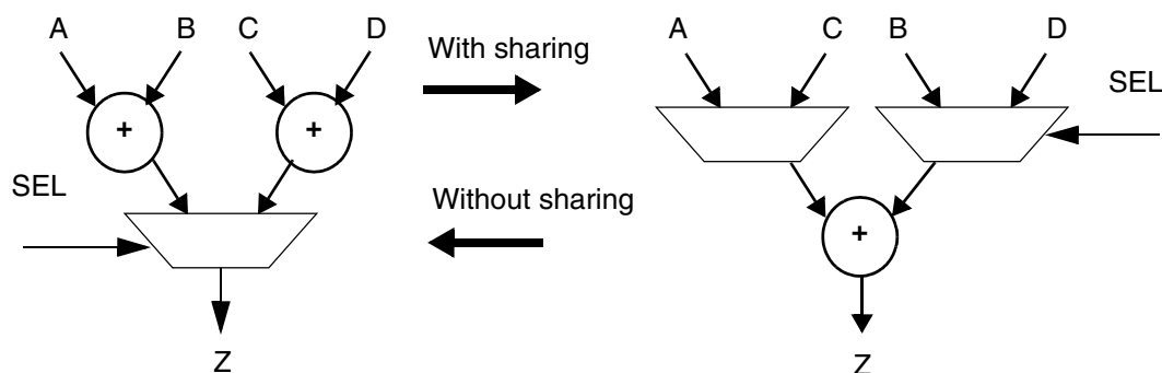
Figure 13-4 Design With and Without Sharing
