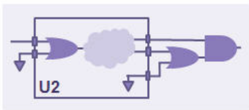
Figure 12-1 Design Before Boundary Optimization
