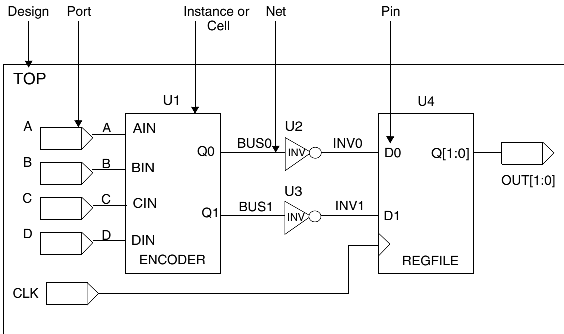
Figure 1-3 Design Objects
