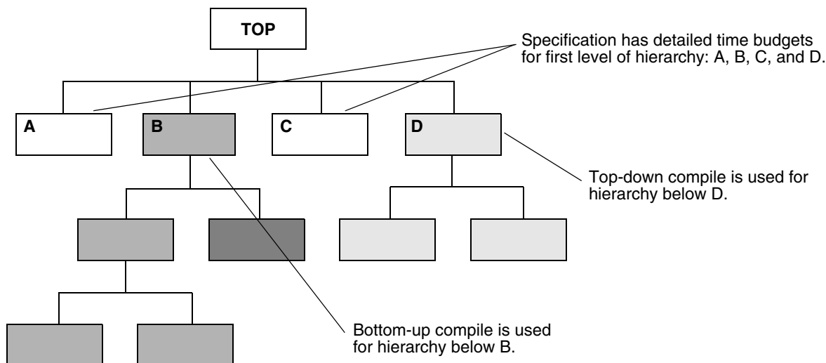
Figure 10-3 Mixing Compilation Strategies
