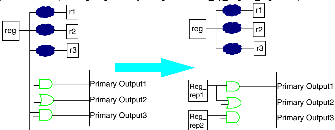
Figure 15-17 Replicating Registers By Using the -driven_by_original_register Option
