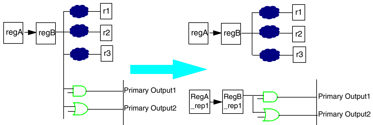
Figure 15-15 Replicating Registers For the Transitive Fanout
