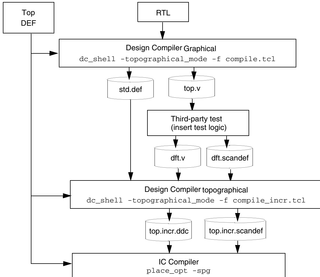
Figure 23-1 Incremental ASCII Physical Guidance Flow With a Third-Party DFT Flow
