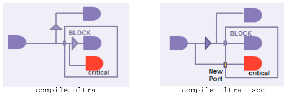
Figure 12-3 Buffering Across the Hierarchy Comparison
