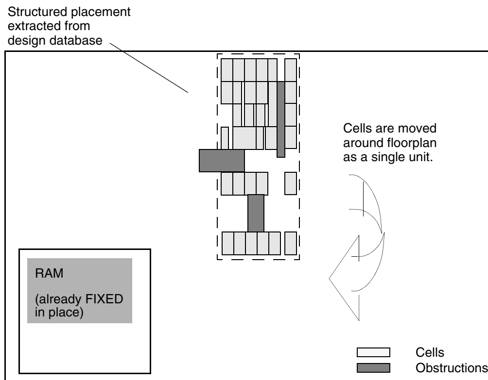
Figure 9-10 Relative Placement in a Floorplan
