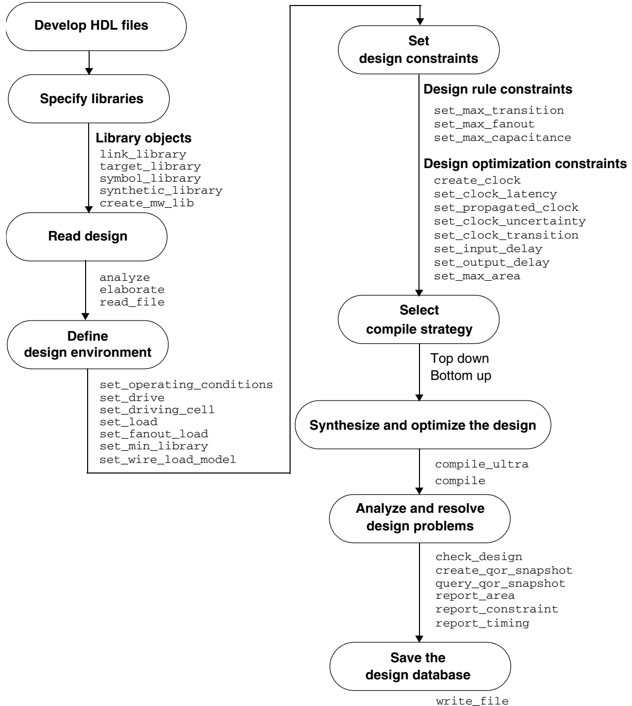
Figure 2-1 Synthesis Flow
